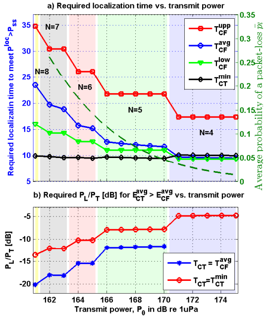
Fig. 5: a) Effect of transmit power on the minimum time required for localization, and the average probability of a packet-loss \bar{p}_l (dashed-line); b) The minimum value of \frac{P_L}{P_T} in dB below which the average energy consumption of CTS is greater than that of CFS.
