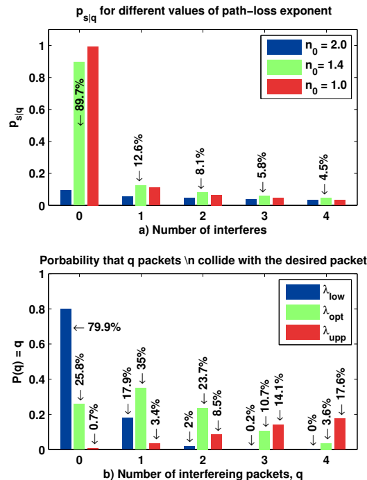
Fig. 4: a) Probability of successful packet reception versus different number of interferers. b) Probability that q interferers collide with the desired packet. For this figure, \lambda_{low} , \lambda_{opt} and \lambda_{upp} are chosen from Fig. 3.
